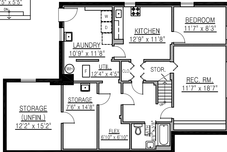
BASEMENT FLOOR PLAN FLOOR AREA: 1,213 sq.ft.
