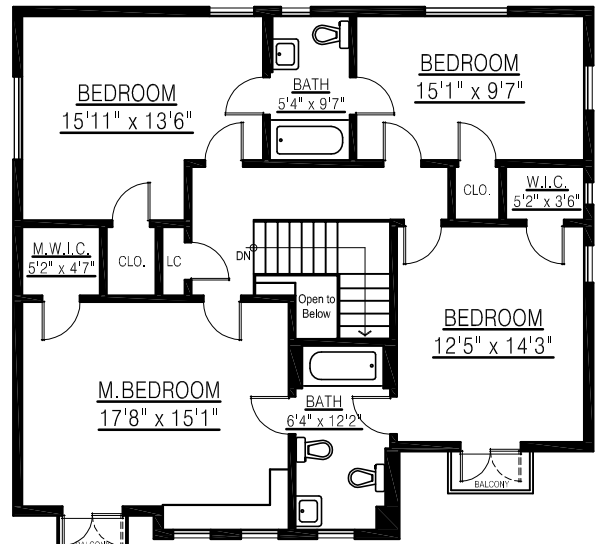
UPPER FLOOR PLAN FLOOR AREA: 1,232 sq.ft.
